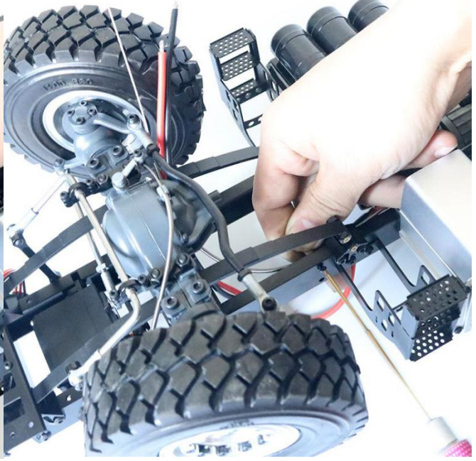
Installation diff locking, general assembly picture (mark for easy adjustment when finishing assembling)
