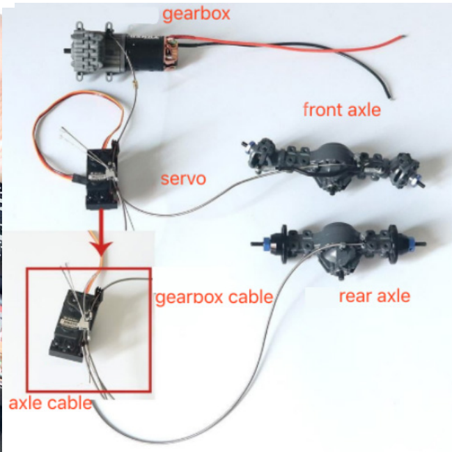
Installation diff locking, general assembly picture (mark for easy adjustment when finishing assembling)
